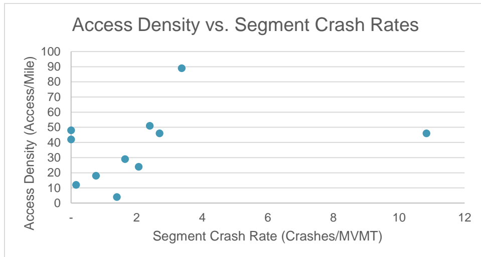
Figure 10. Scatter Plot of Access Density vs. Segment Crash Rates
