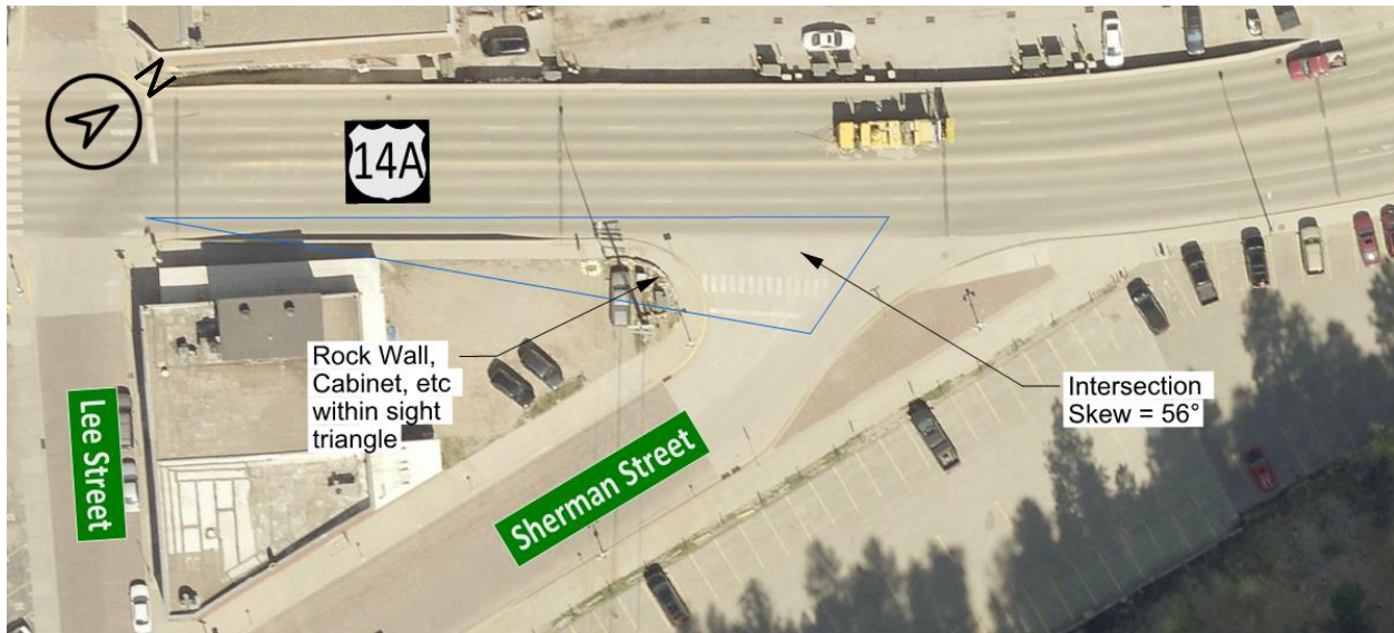
Figure 16. Intersection Geometrics at US14A and Sherman Street
