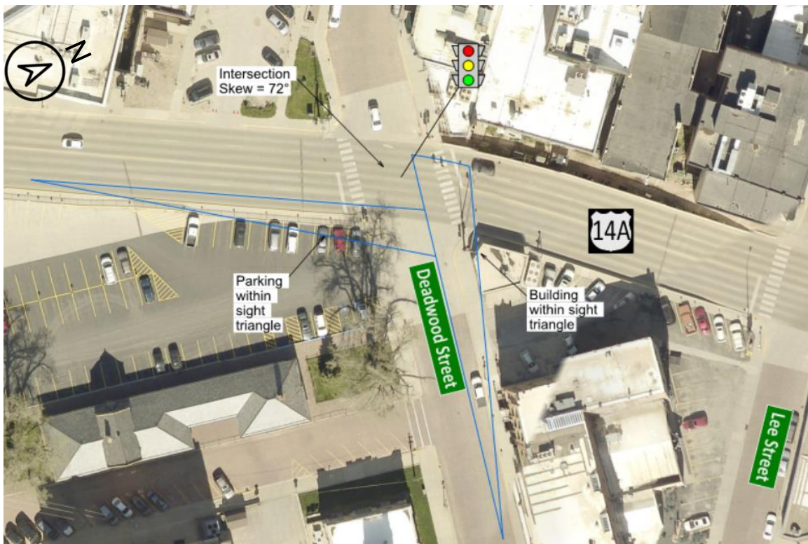
Figure 14. Intersection Geometrics at US14A and Deadwood Street
