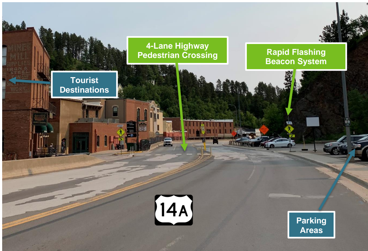
Figure 20. Crosswalk with Rapid Flashing Beacon across US14A at Wall Street
