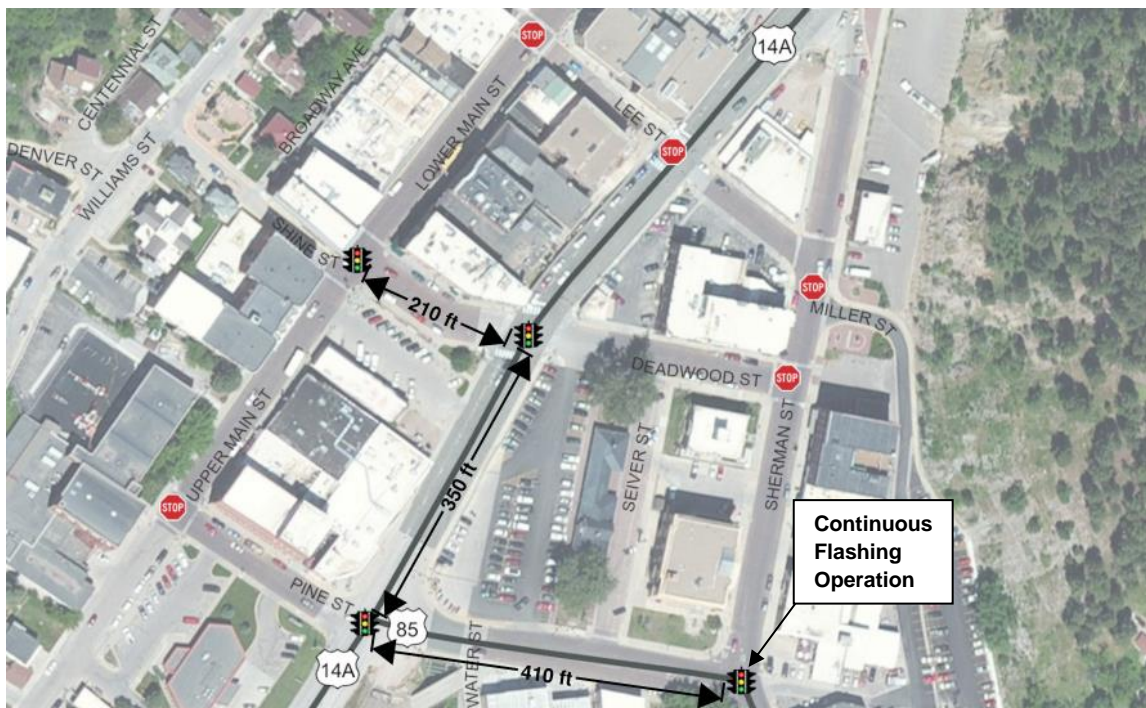
Figure 7. Spacing of Signals in Deadwood's Downtown Core
